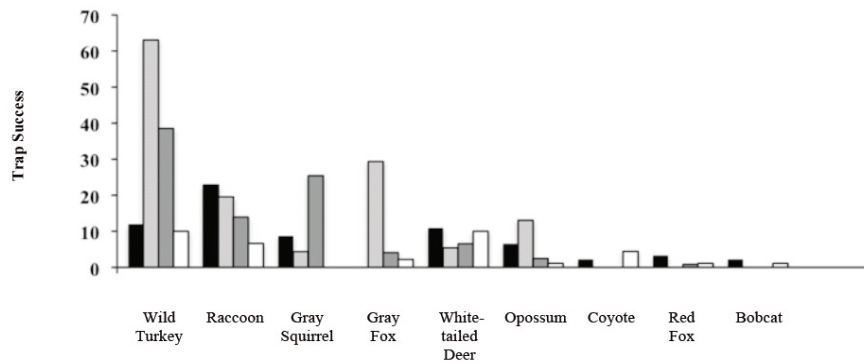
FIGURE 3. Trap success for each target species as a function of season. Spring (black bar) months were March, April, and May. Summer (light gray bar) months were June, July, and August. Fall (dark gray bar) months were September, October, and November. Winter (white bar) months were December, January, and February.
